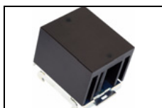
HS-01: 47 x 58 x 53 (h) HS-01 + SSR: 47 x 58 x 90 (h)
