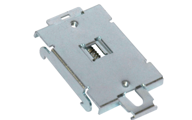
Dimensions: 77x44x14(h)mm
