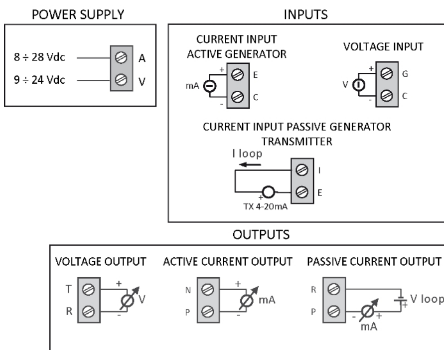
Figure 2- Connections
