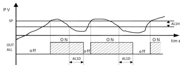
Example with "FUNC ALL1" = HiEd (relative maximum value alarm)
