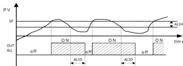
Example with "FUNC ALL1" = HidE (relative maximum value alarm)
