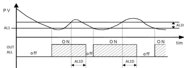
Operation example "FUNC ALL1" = Loab (minimum value alarm)
