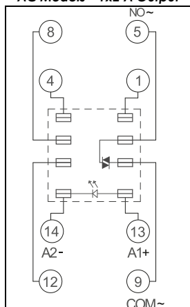
Modelli in AC - Uscita 1x2 A AC Models - 1x2 A Output
