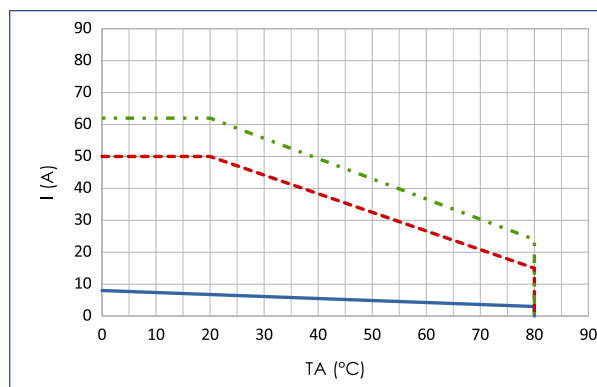
SSR39 80 A
